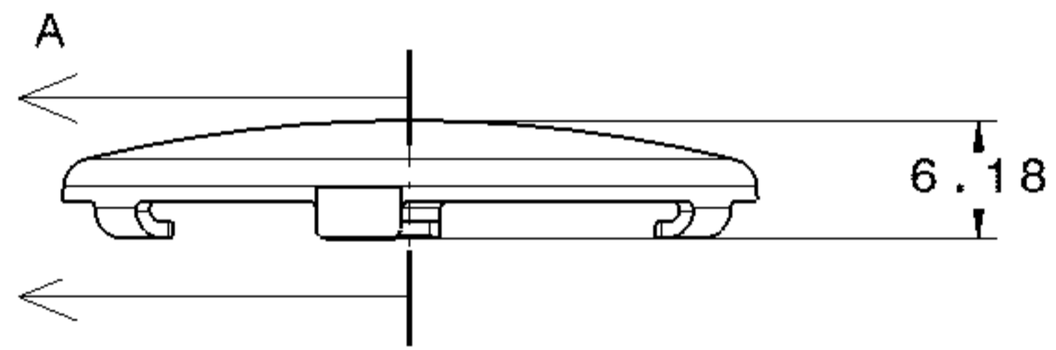
Front view Scale: 2:1
