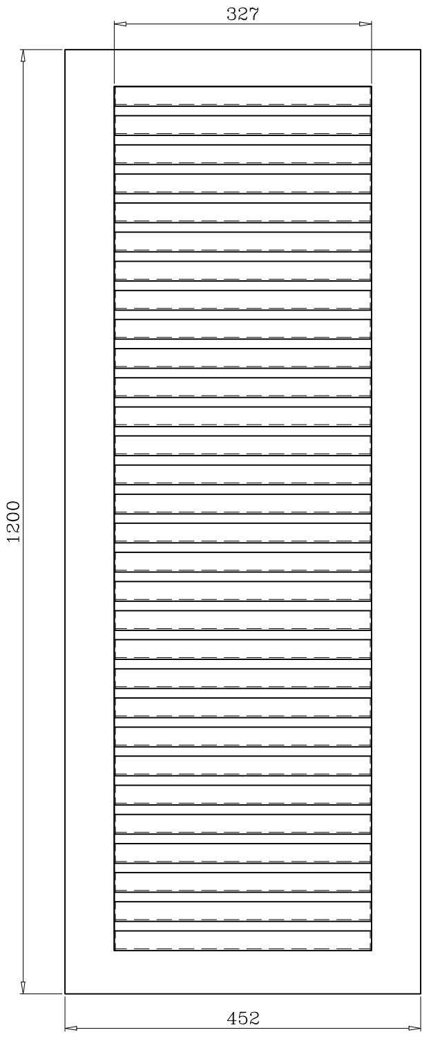
FRONT VIEW
