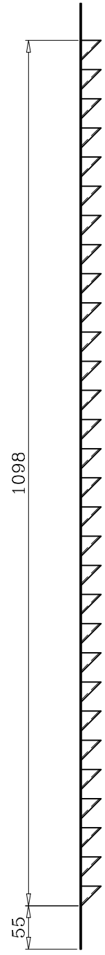
SIDE VIEW
